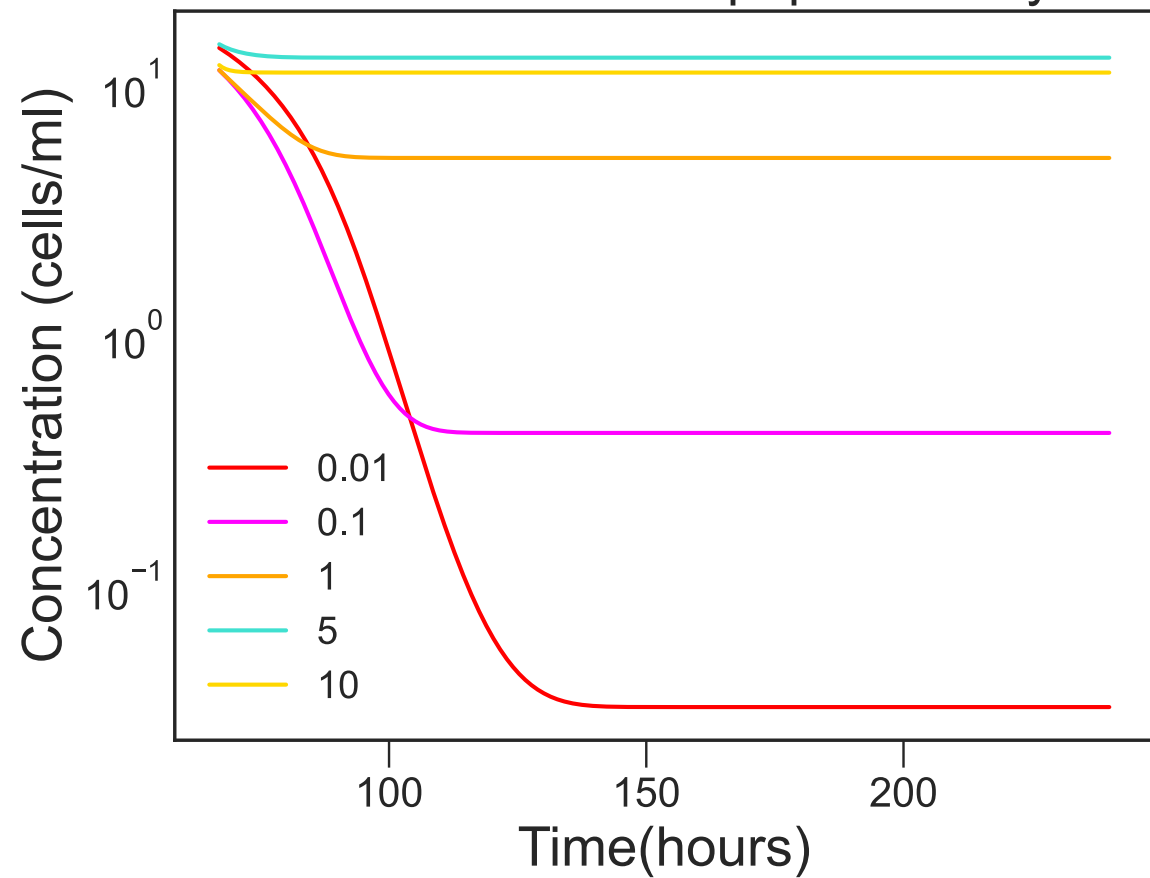
Simulated Sal. ruber M1 population dynamics
