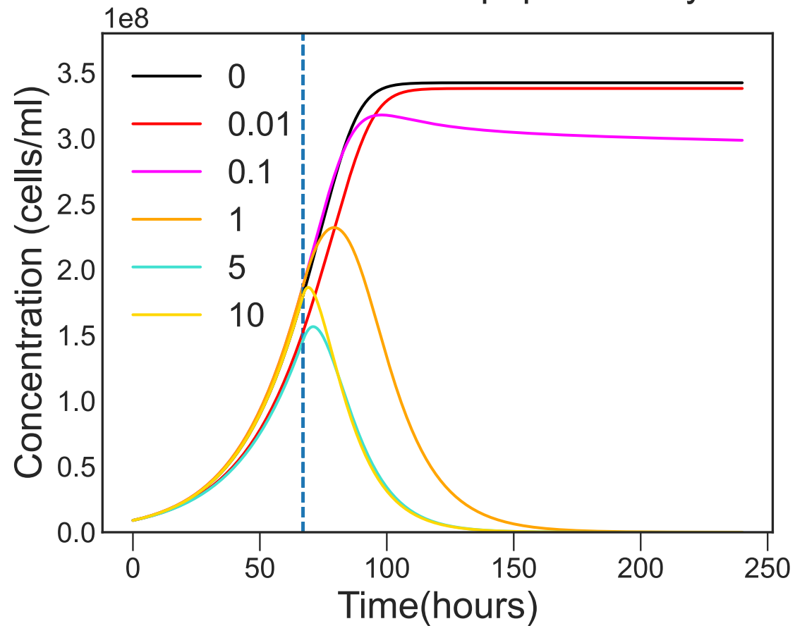
Simulated Sal. ruber M1 population dynamics
